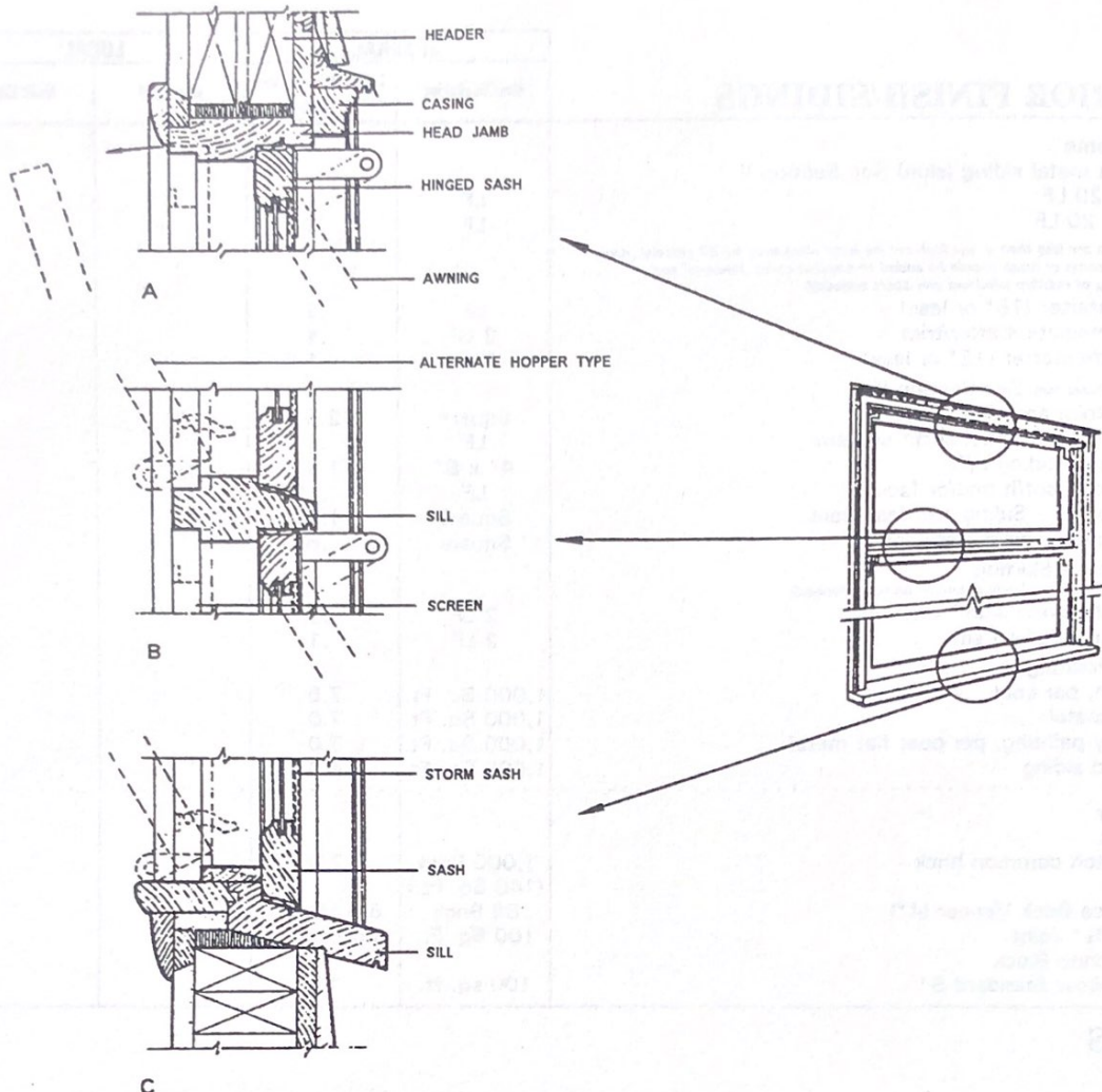
Awning window. Cross sections: A, Head jamb; B, horizontal mullion; C, sill
