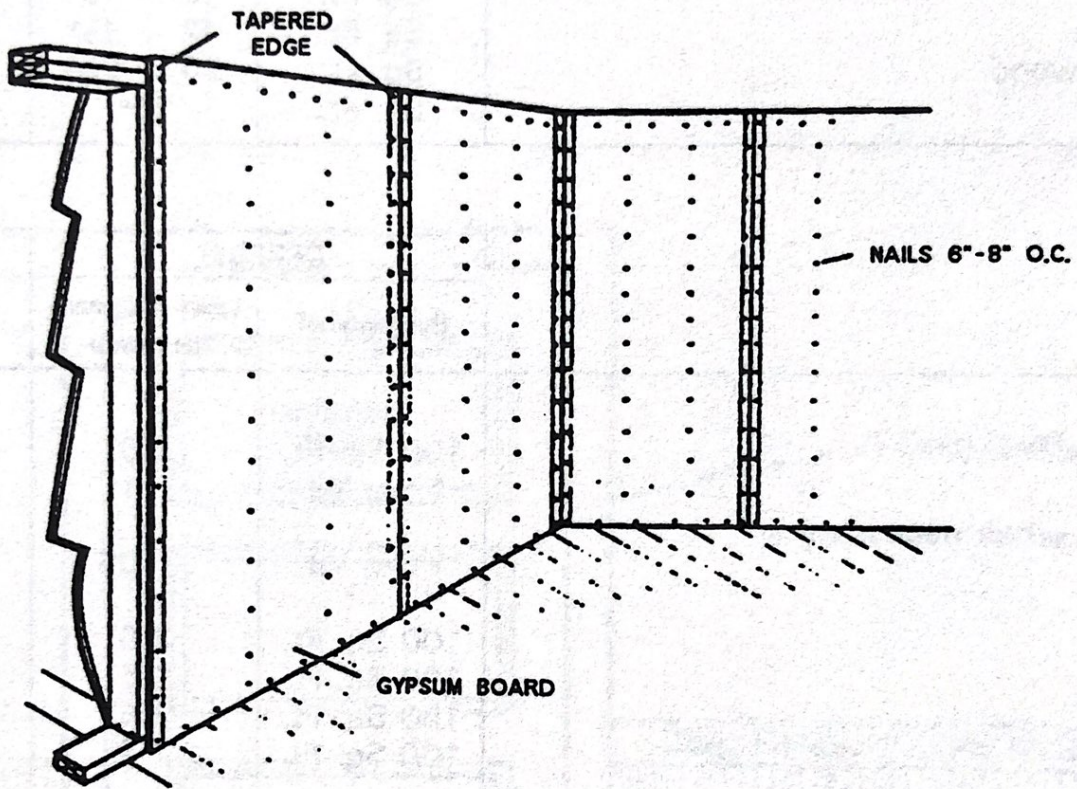
Application of gypsum board finish.
