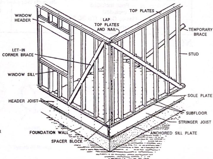
Wall framing used with platform construction.
