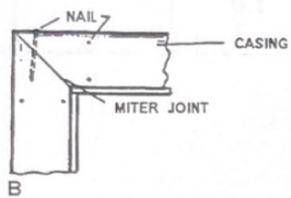
Doorframe and trim: A, Installation; B, miter joint for casing.
