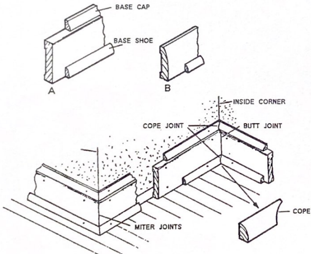
Base molding: A, Square-edge base; B, narrow ranch base;
