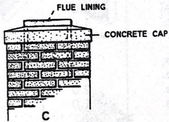
Chimney details: A, Spacer between flues; B, height of chimneys; C, chimney cap. D, metal double wall chimney; E, metal single wall chimney & cap
