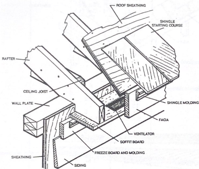
Narrow Box Cornice.
