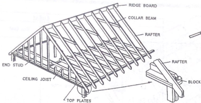
Ceiling and roof framing - overall view of gable roof framing.
