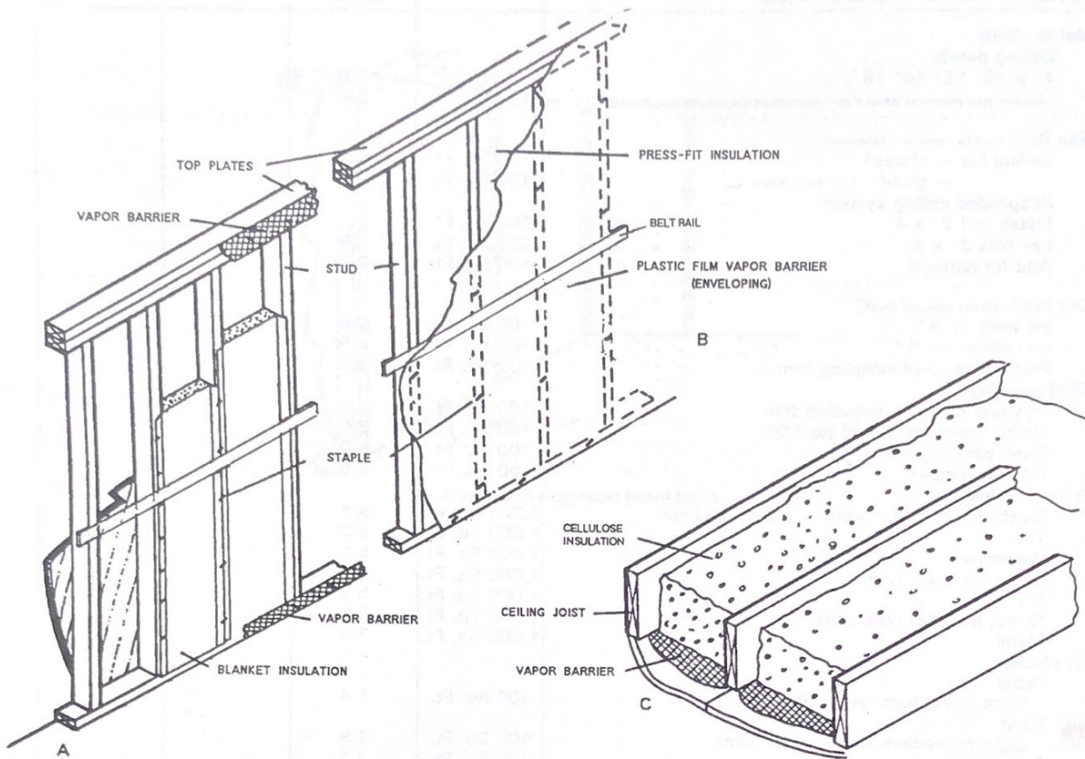
Application of insulation: A, Wall section with blanket type; B, wall section with "press-fit" insulation; C, ceiling with full insulation.
