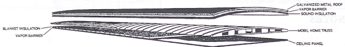
Mobile home roof structure.
