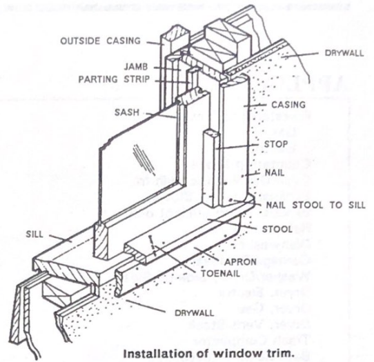
Installation of window trim.
