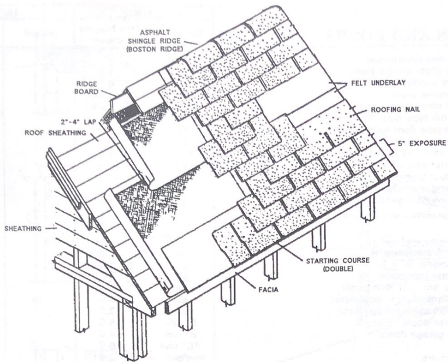
Application of asphalt shingles.
